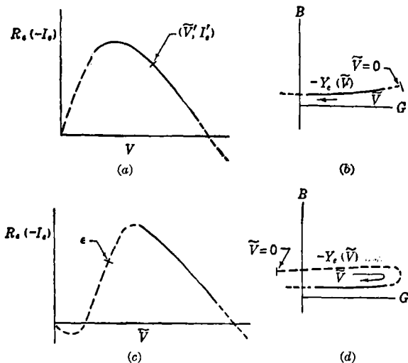
FIG. 7-13.—(a), (c) The real component of the electronic current \bar{I}_e plotted vs. the a-c voltage \bar{V} ; (b), (d) the operating curves corresponding to Fig. 7-13a and c.
